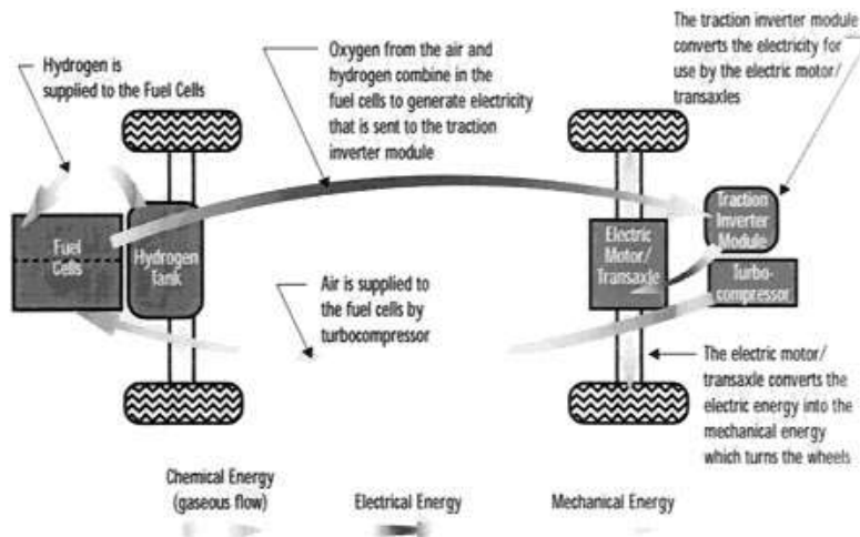
Figure 10. The P2000, a Ford Motor company design of a vehicle using a direct hydrogen polymer electrolyte fuel cell.
