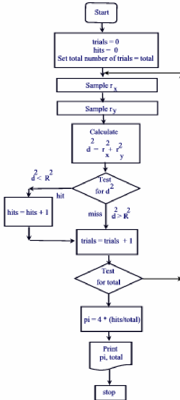
Fig.3: Flow Chart for dart throwing problem.
