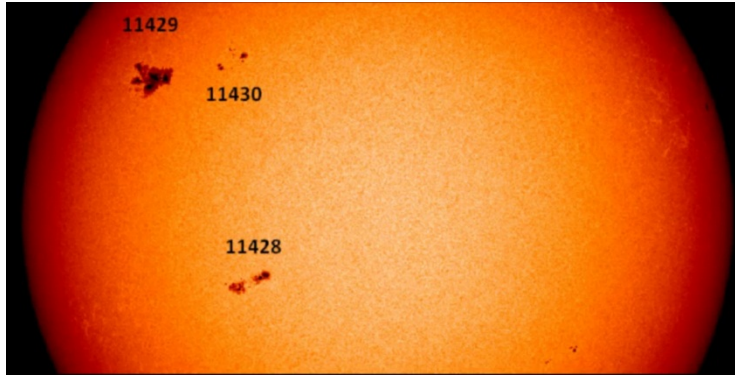
Figure 15. Solar flare visual picture on March 5, 2012 at the 11429 location. Source: NOAA.
