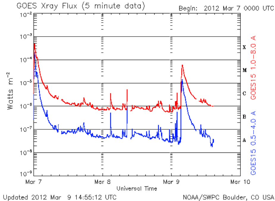
Figure 17. Plot showing three days of 5-minute solar x-ray flux values measured on the SWPC primary GOES satellite. One low value may appear prior to eclipse periods. Source: NOAA.
