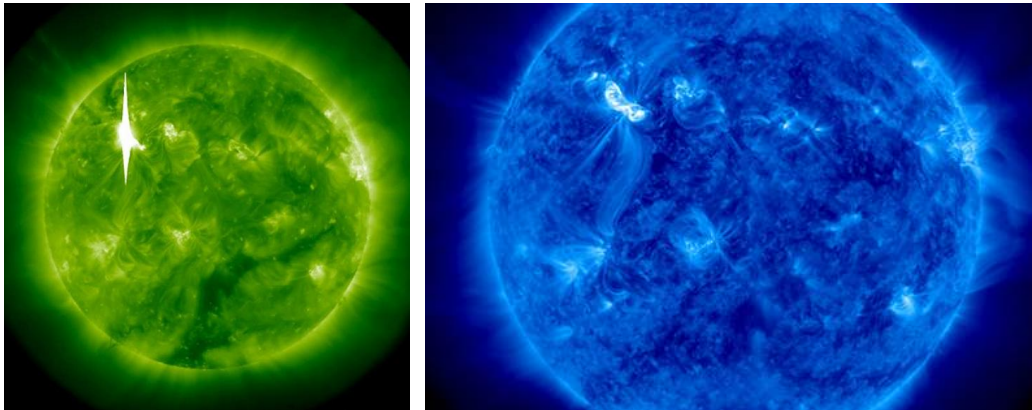
Figure 16. Infrared and x-ray pictures of the March 5, 2012, showing onset of the Coronal Mass Ejection. Source: NOAA.
