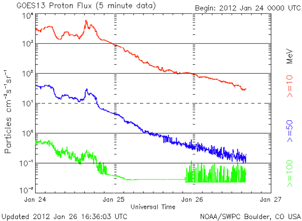
Figure 10. GOES Satellite 5-minute averaged integral proton flux (protons/cm 2 -s-sr) as measured by the SWPC primary GOES satellite for energy thresholds of \geq 10 , \geq 50 , and \geq 100 MeV. SWPC's proton event threshold is 10 protons/cm 2 -s-sr at \geq 10 MeV. Large particle fluxes have been associated with satellite single event upsets (SEUs). Source: NOAA.
