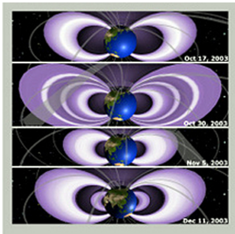
Figure 20. Solar storms effects on the Earth's protective Van Allen magnetic fields. Source: NASA.
