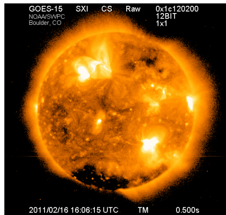
Figure 14. Solar storm on February 16, 2011. Source: NOAA.
