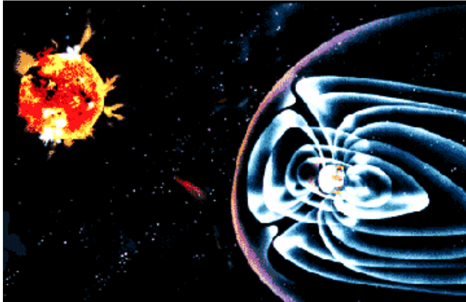
Fig. 17: The Earth's magnetic field interacts with the solar wind and with coronal mass ejections, trapping the generated particles.
