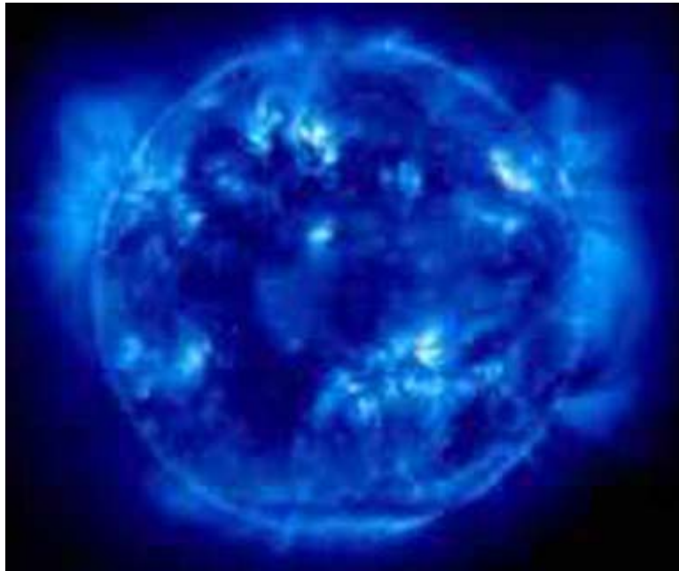
Fig. 14: Sun magnetic prominences caused by local magnetic fields disruptions.
