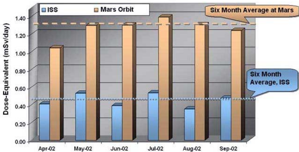
Fig. 10: Comparison of effective dose rate or dose equivalent rate for a six months mission in International Space Station (ISS) and in a Mars Orbit.
