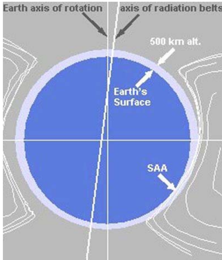
Fig. 18: The South Atlantic Anomaly (SAA) occurs because of the asymmetry of the axis of rotation of the Earth and its magnetic field axis.
