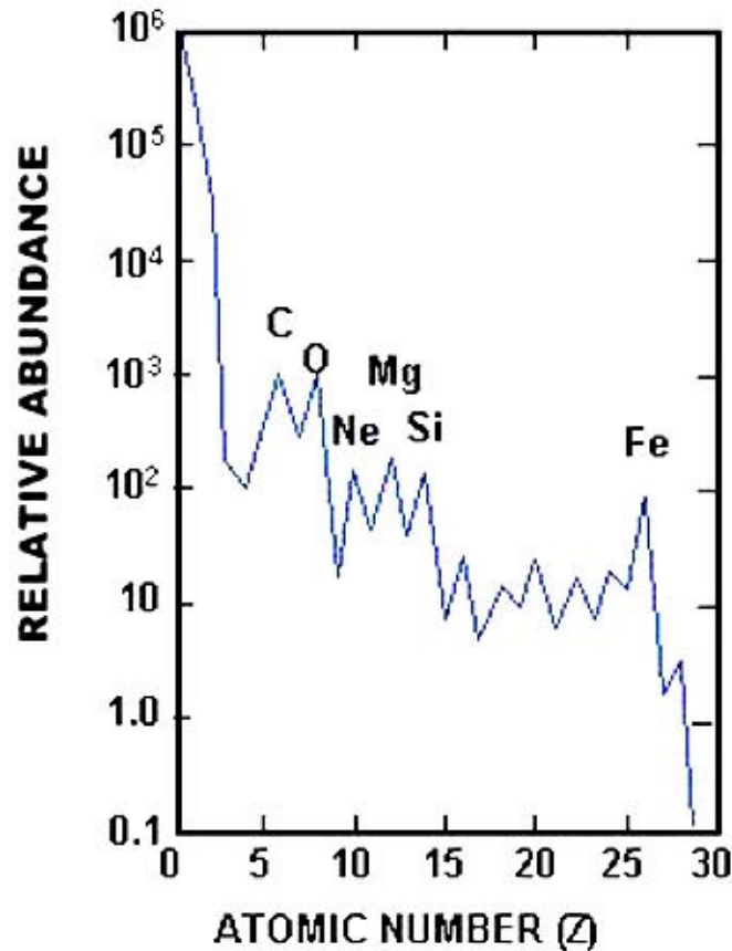
Fig. 12: Logarithmic relative abundances of space particles.
