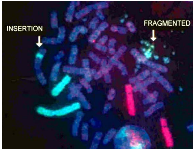
Fig. 9: Damaged metaphase chromosome number 2, post a space flight.
