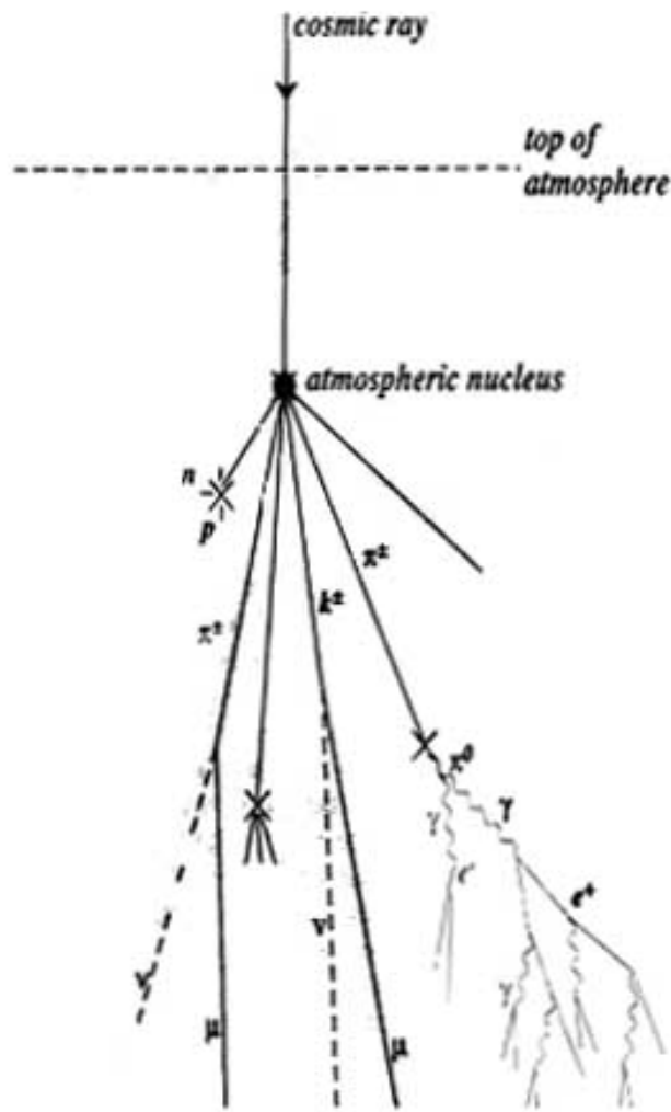
Fig. 6: Components of a cosmic ray shower in the atmosphere.
