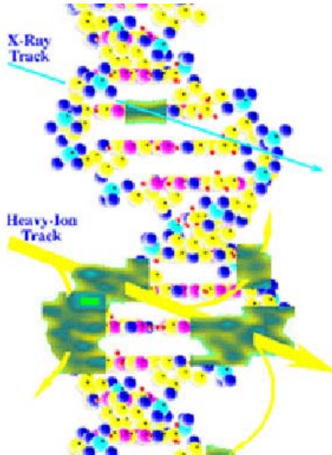
Fig. 8: Comparison of effect of an x-ray photon and a heavy ion on the DNA molecule.
