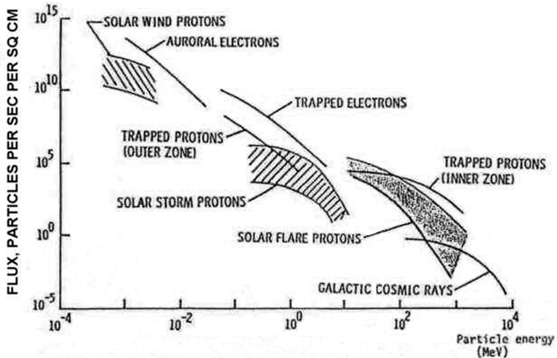
Fig. 11: Types of space radiation and their fluxes.
