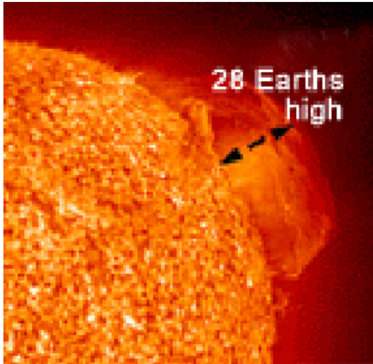
Fig. 16: Coronal Mass Ejection recorded in 1997 by the SOHO satellite.
