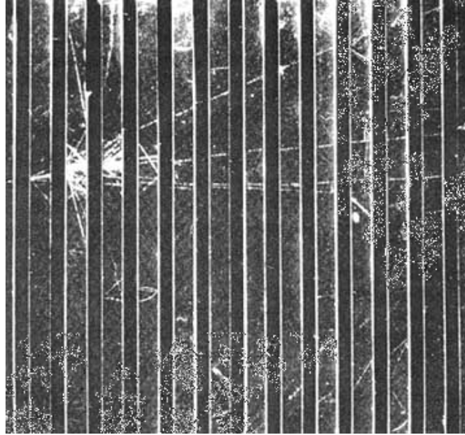
Fig. 4: Cloud chamber photograph of a nuclear disintegration resulting from a cosmic ray collision.
