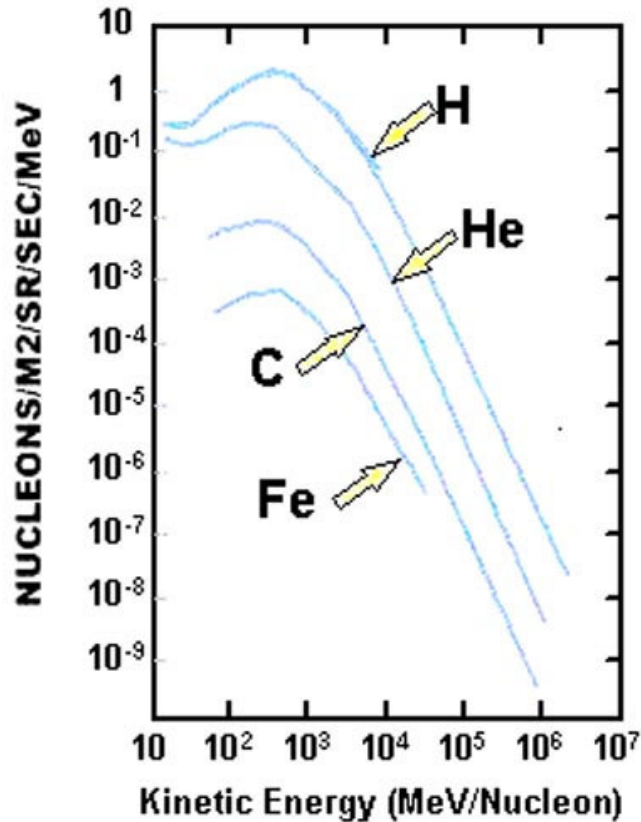
Fig. 13: Logarithmic energy distribution of HZE particles.
