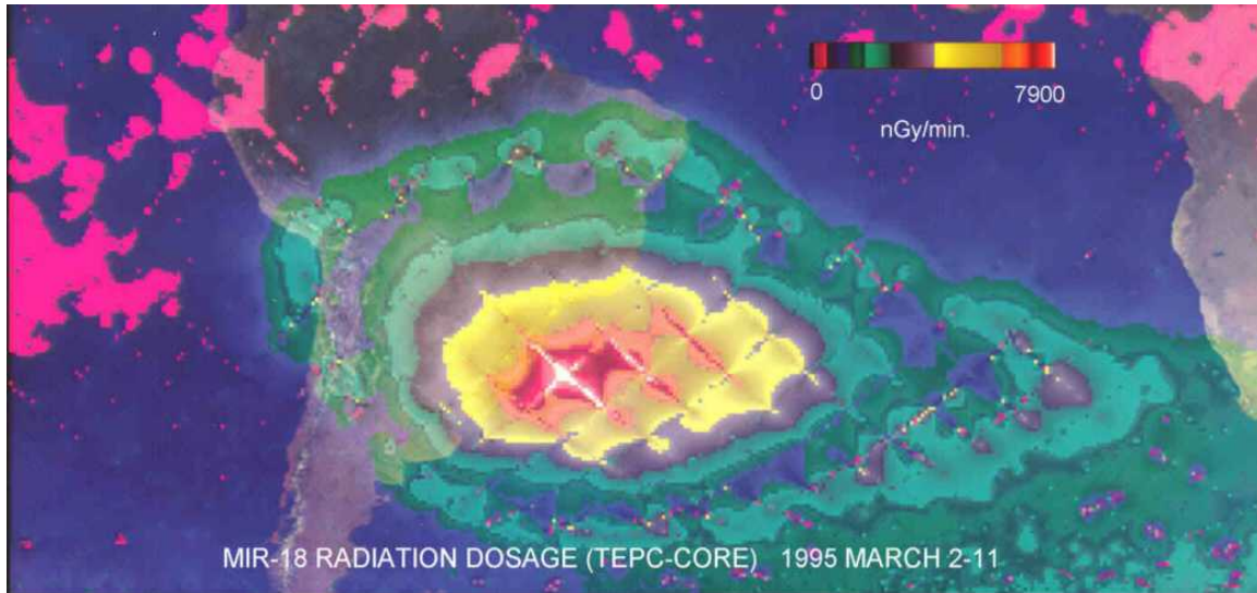
Fig. 19: Dose rate to the MIR-18 Space Station showing the South Atlantic Anomaly just east of the Brazilian coastline.
