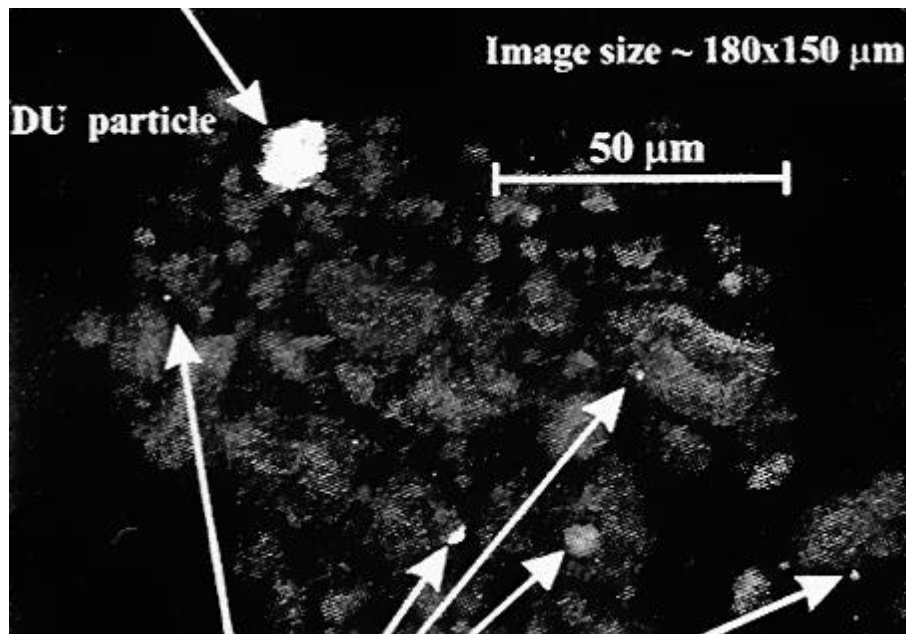
Figure 13. Depleted uranium particles can be detected in contaminated soil using a Scanning Electron Microscope (SEM) that is equipped with an Energy Dispersive X-ray Fluorescence detector.
