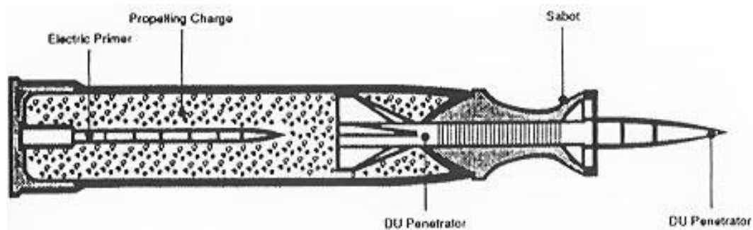
Figure 4. Schematic of a sabot armor piercing round with a depleted uranium penetrator.
