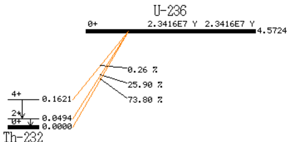
Figure 2. Alpha decay scheme of \text{U}^{236} . Source: Chart of the Nuclides.
