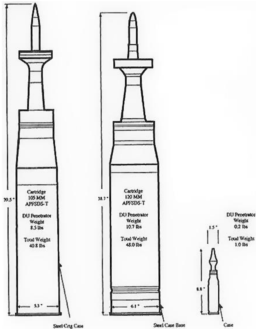
Figure 8. Depleted uranium cartridges of different sizes and weights.
