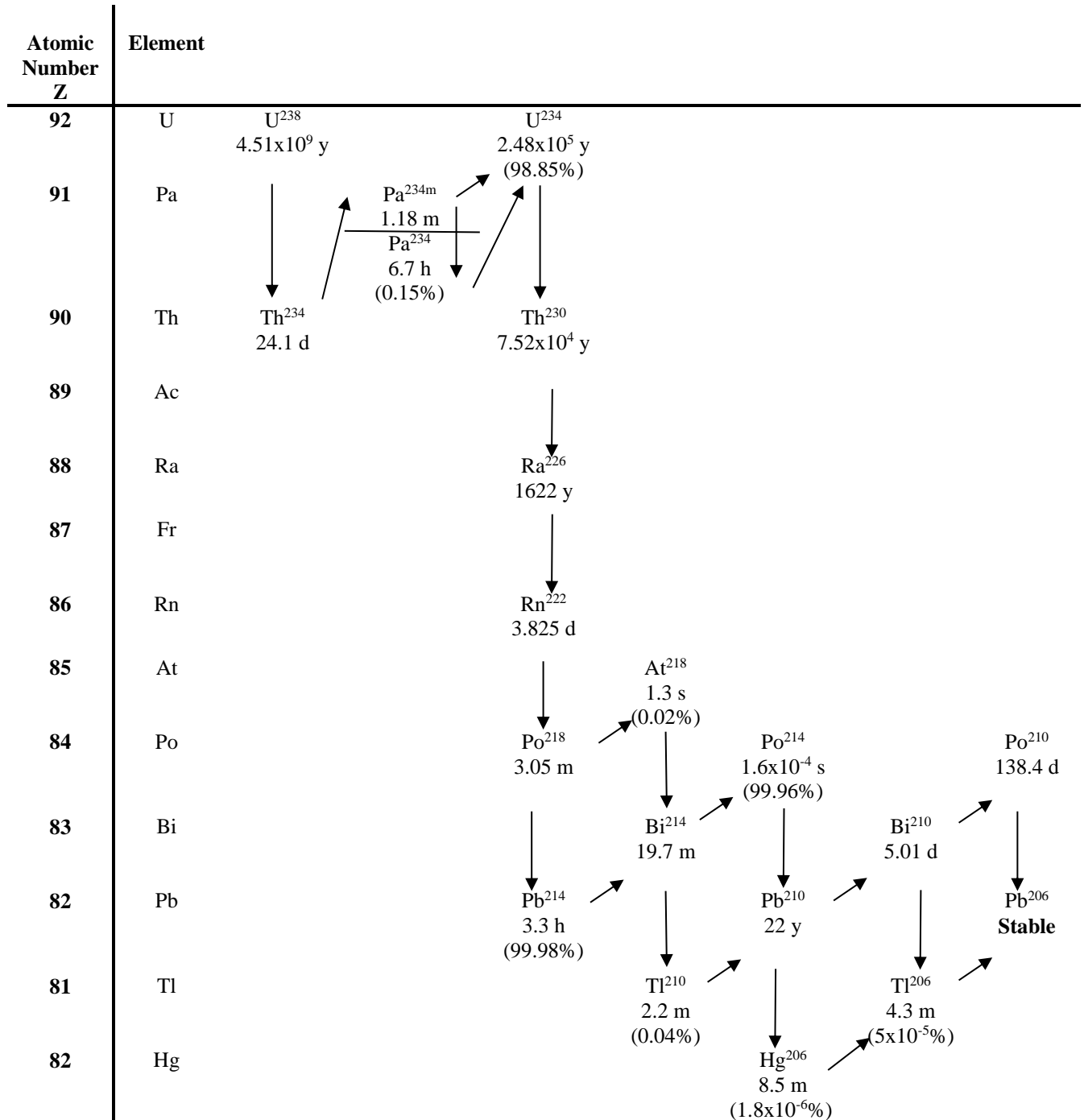
Figure 11. The U^{238} ( 4n+2 ) radioactive decay chain.
