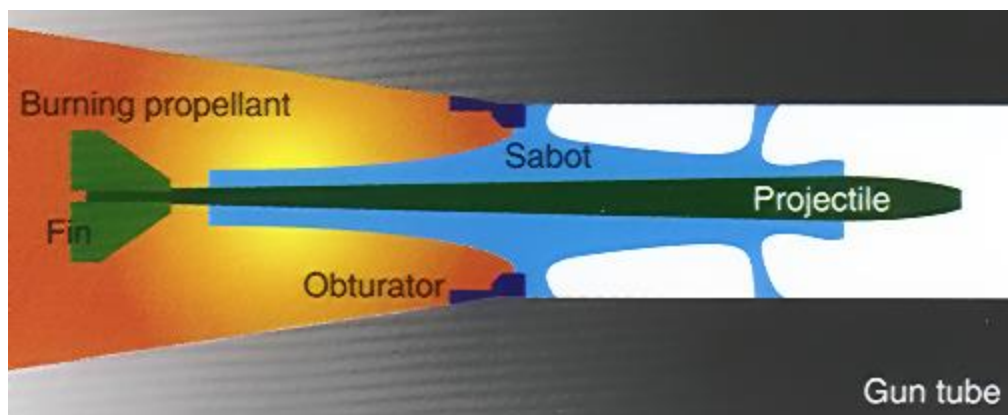
Figure 6. Cross Section of sabot showing kinetic energy transfer from the propellant to the sabot.
